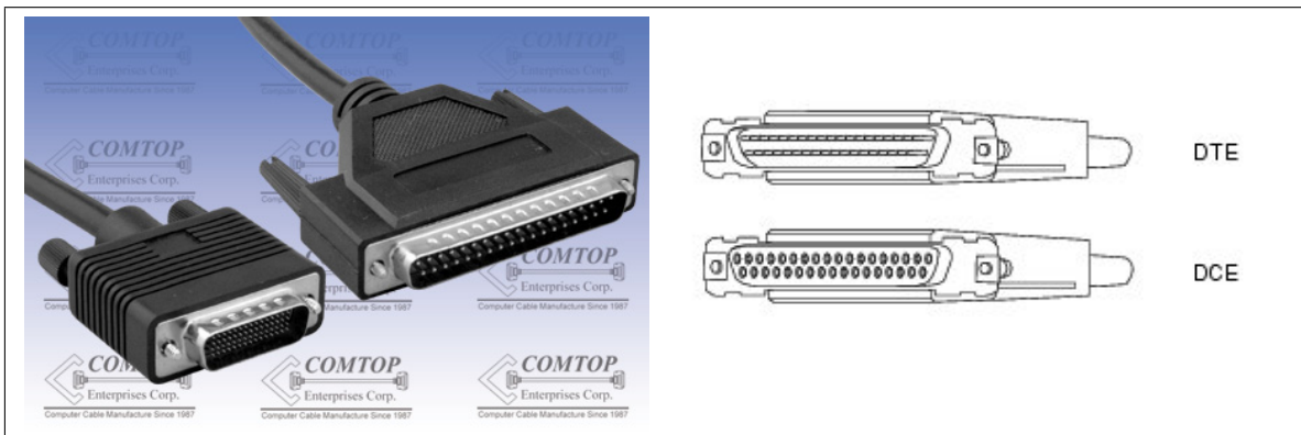
Figure 2: Connector type (standard): HD-60 (m) to DB-37 (EIA/TIA-449)
