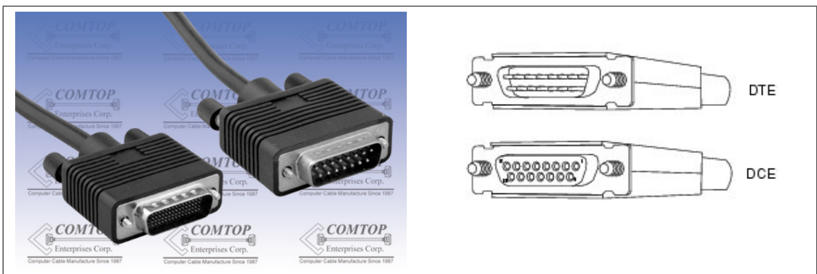
Figure 5: Connector type (standard): HD-60 (m) to DB-15 (X.21)
