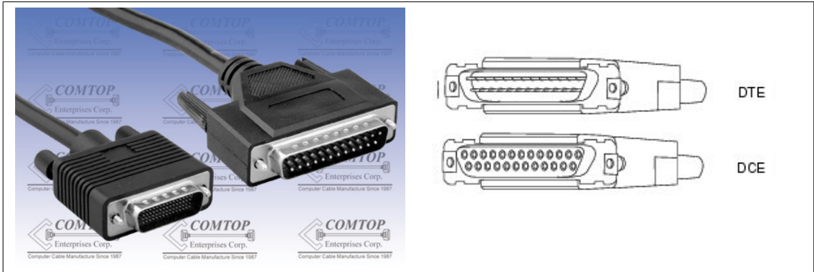
Figure 3: Connector type (standard): HD-60 (m) to DB-25 (EIA/TIA-530)
