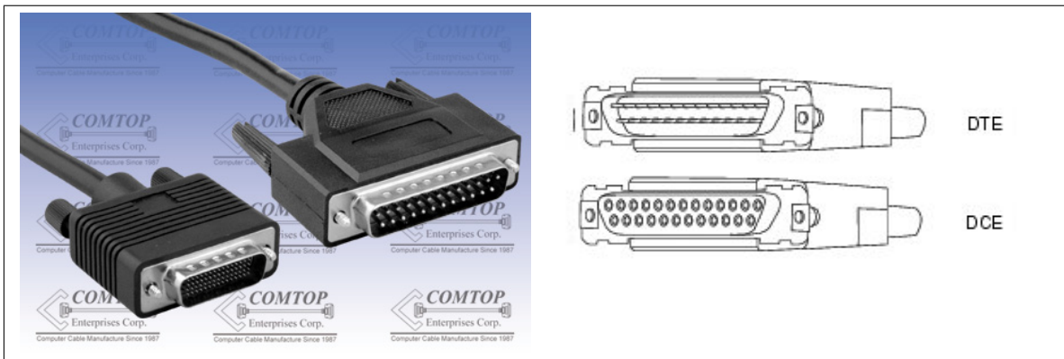
Figure 1: Connector type (standard): HD-60 (m) to DB-25 (EIA/TIA-232)
