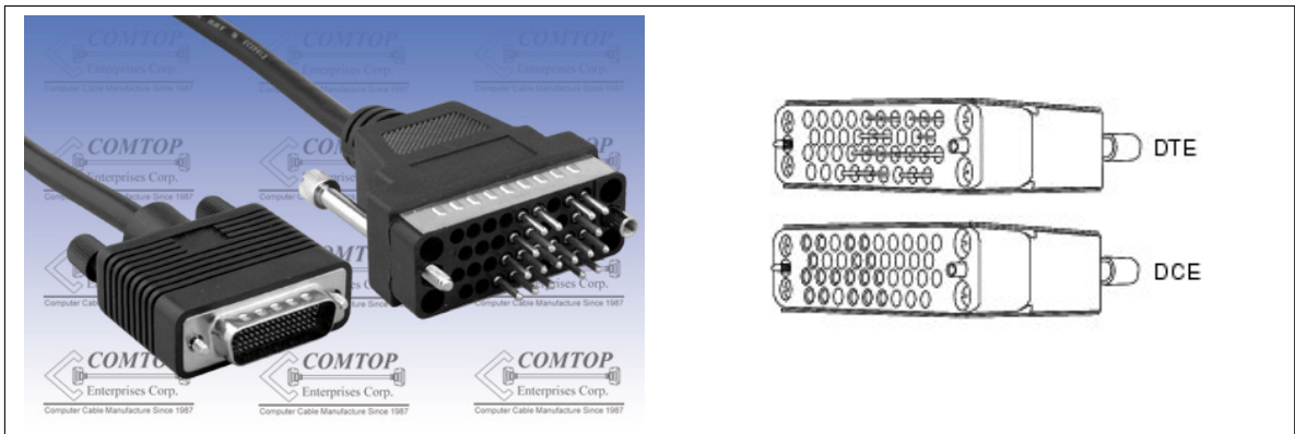
Figure 4: Connector type (standard): HD-60 (m) to 34-pin Winchester-type (V.35)
